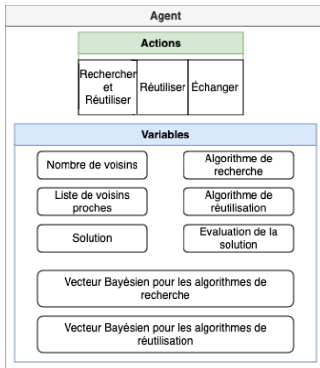
FIGURE 6.10 – Structure interne des agents.
